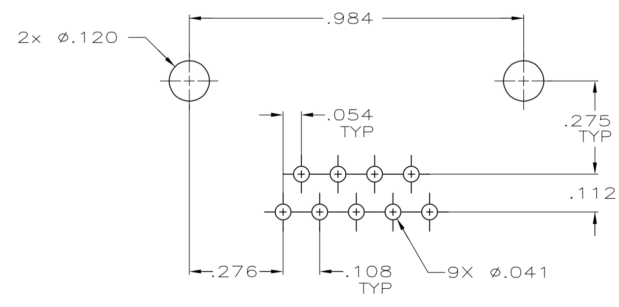
P.C. BOARD MOUNTING DIMENSIONS \Delta
